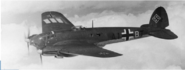
Heinkel 111 P = 2 x 1350CV Vmax = 435km/h Plafond = 8500m Charge utile = 2000kg
